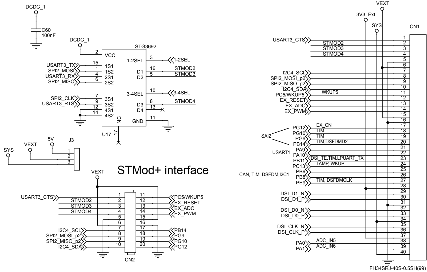
Figure 4. STEVAL-STWINKT1B schematic (2 of 7)
