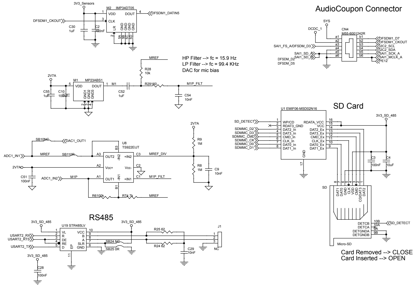
Figure 7. STEVAL-STWINKT1B schematic (5 of 7)
